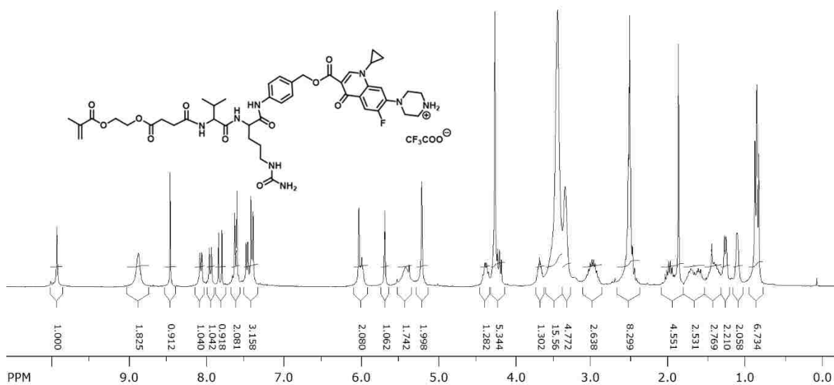
Figure S4. ^1\text{H-NMR} spectrum of cathepsin B cleavable monomer SMA-Val-Cit-PAB-ciprofloxacin ( 11 )
