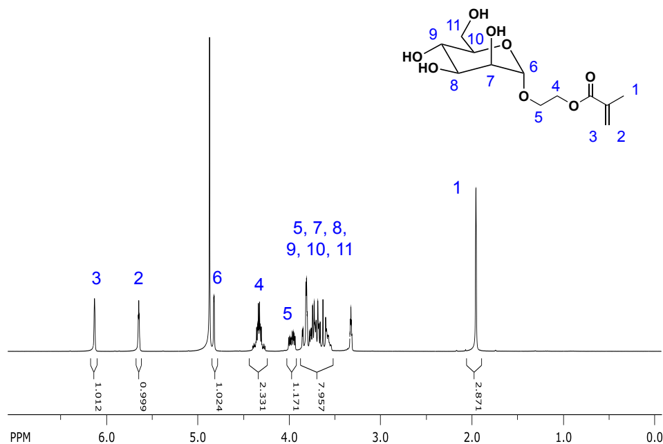
Figure 3.14. ^1\text{H} NMR spectrum of 2-O-( \alpha -D-mannosyl)hydroxyethyl methacrylate. Proton NMR scans were conducted in MeOD- d_4 at 300 MHz. Successful preparation of the indicated chemical structure was confirmed by the appearance of resonances associated with 2-hydroxyethyl methacrylate (1-5) and mannose (6-11).
